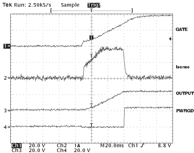
Figure 2. Power-Up Waveforms
